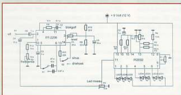
Schema toongenerator
